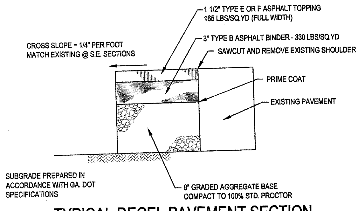
TYPICAL DECEL PAVEMENT SECTION N.T.S.
