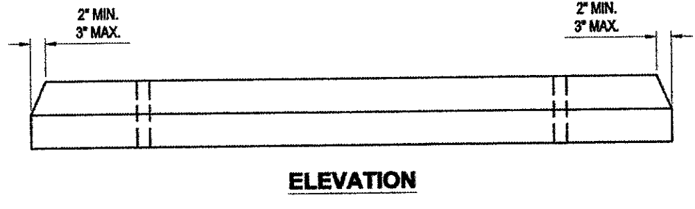
WHEEL STOP DETAIL NOT TO SCALE
